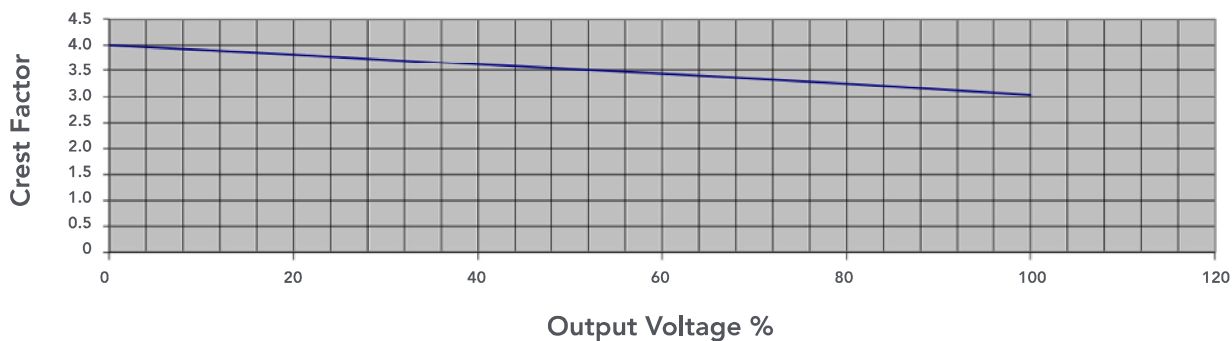
Crest Factor vs Output Voltage %
